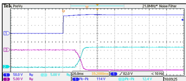
Typical Input/Output Start-Up Characteristic at Full Load
