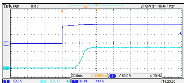
Typical Input/Output Start-Up Characteristic at Full Load
